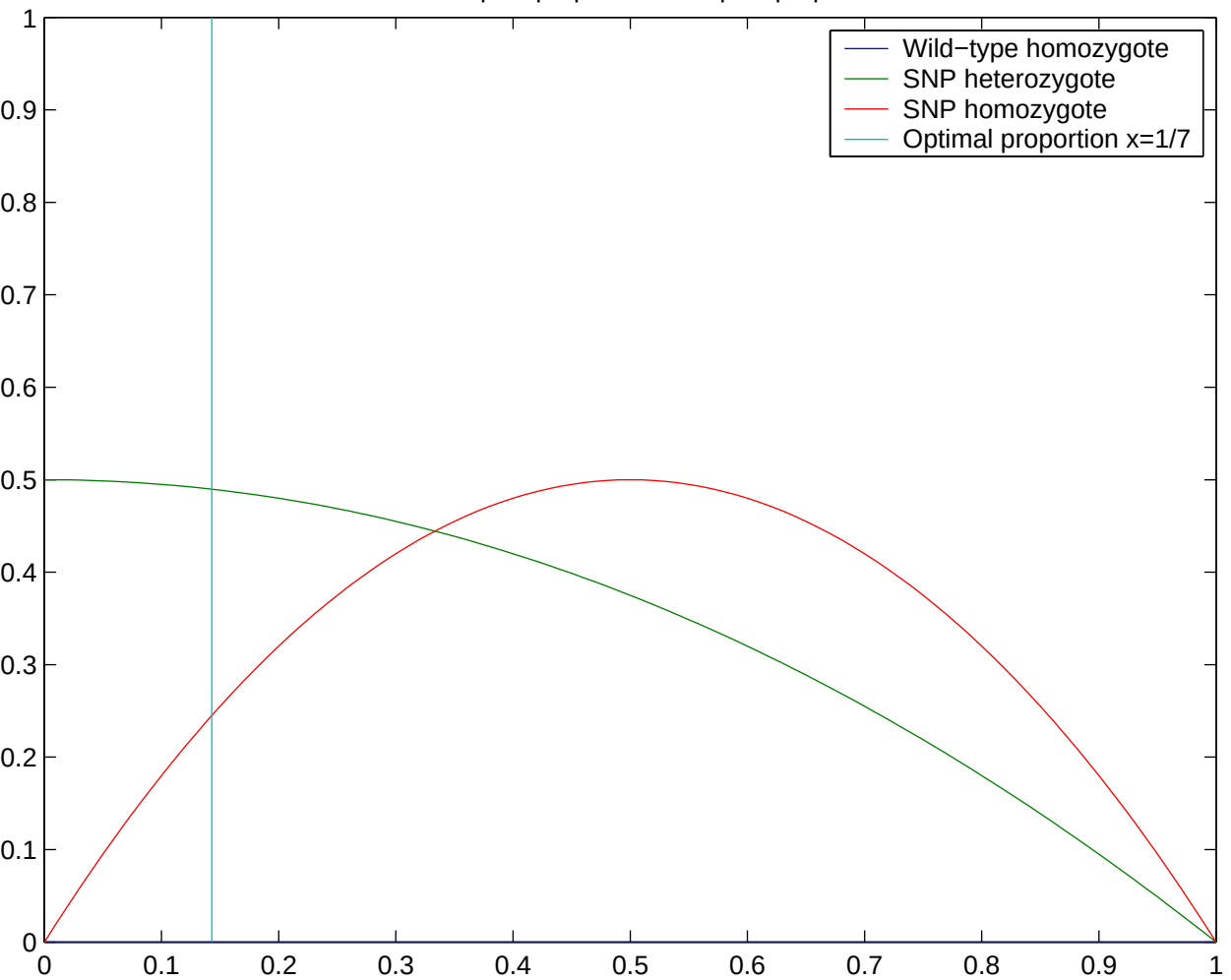
Heteroduplex proportion vs. Spike proportion
