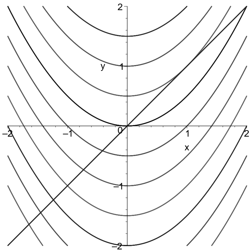
Figure 2. Antiderivatives y(x) = \frac{x^2}{2} + C of f(x) = x .
