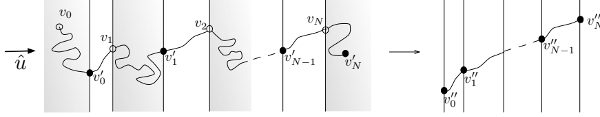
Fig. 3.3 Illustration of the construction. The shaded bad slabs of environments are deleted. The white good slabs are joined together and shifted so that the good path segments connect. So for example points v_1 and v'_1 on the left are identified as v''_1 on the right.
