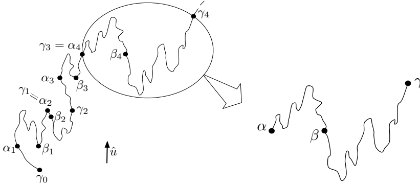
Fig. 3.2 Illustration of the stopping times \alpha_i , \beta_i , and \gamma_i . Note how the immediate backtracking at \gamma_1 makes \alpha_2 = \gamma_1 and \beta_2 = \alpha_2 + 1 .
