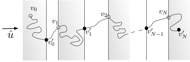
Fig. 3.1 Path segments in shaded regions are bad, the other segments are good. v_i = X_{s_i} and v'_i = X_{s'_i} . Steps going up and to the right represent steps in \mathcal{R}_0 .
